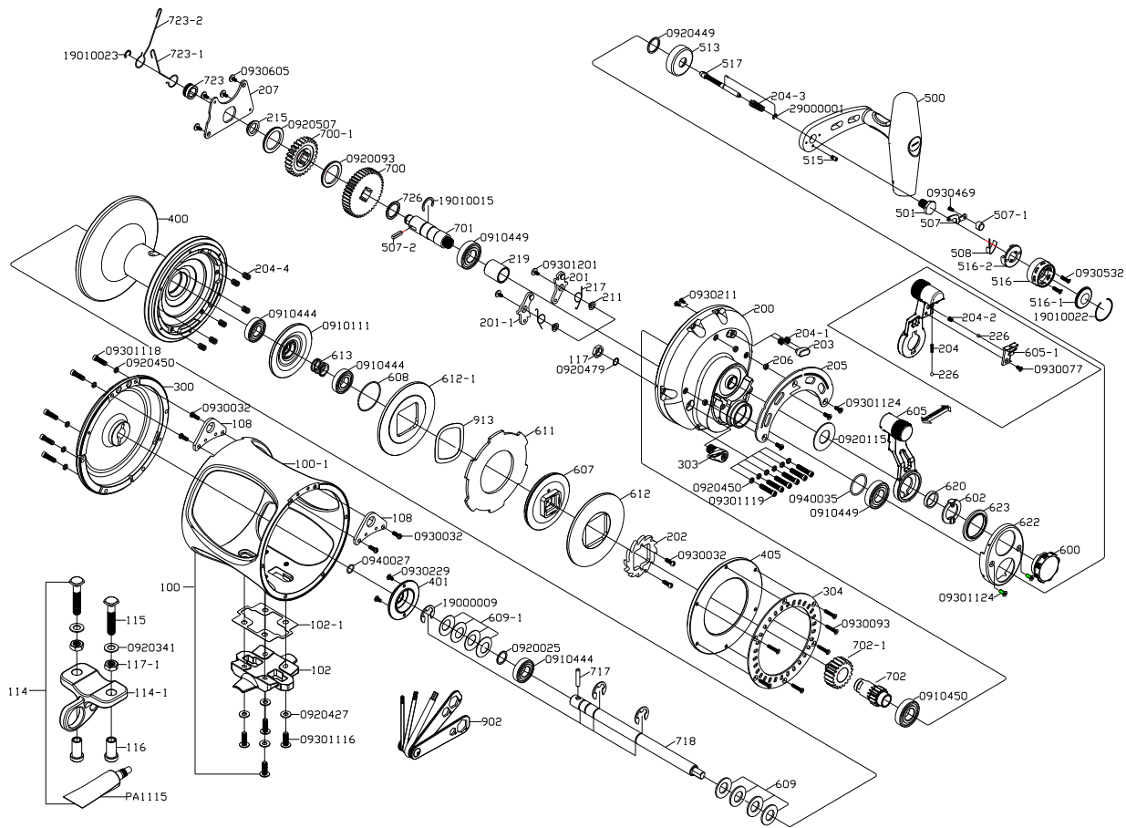
Makaira-80W-2 PART LIST
