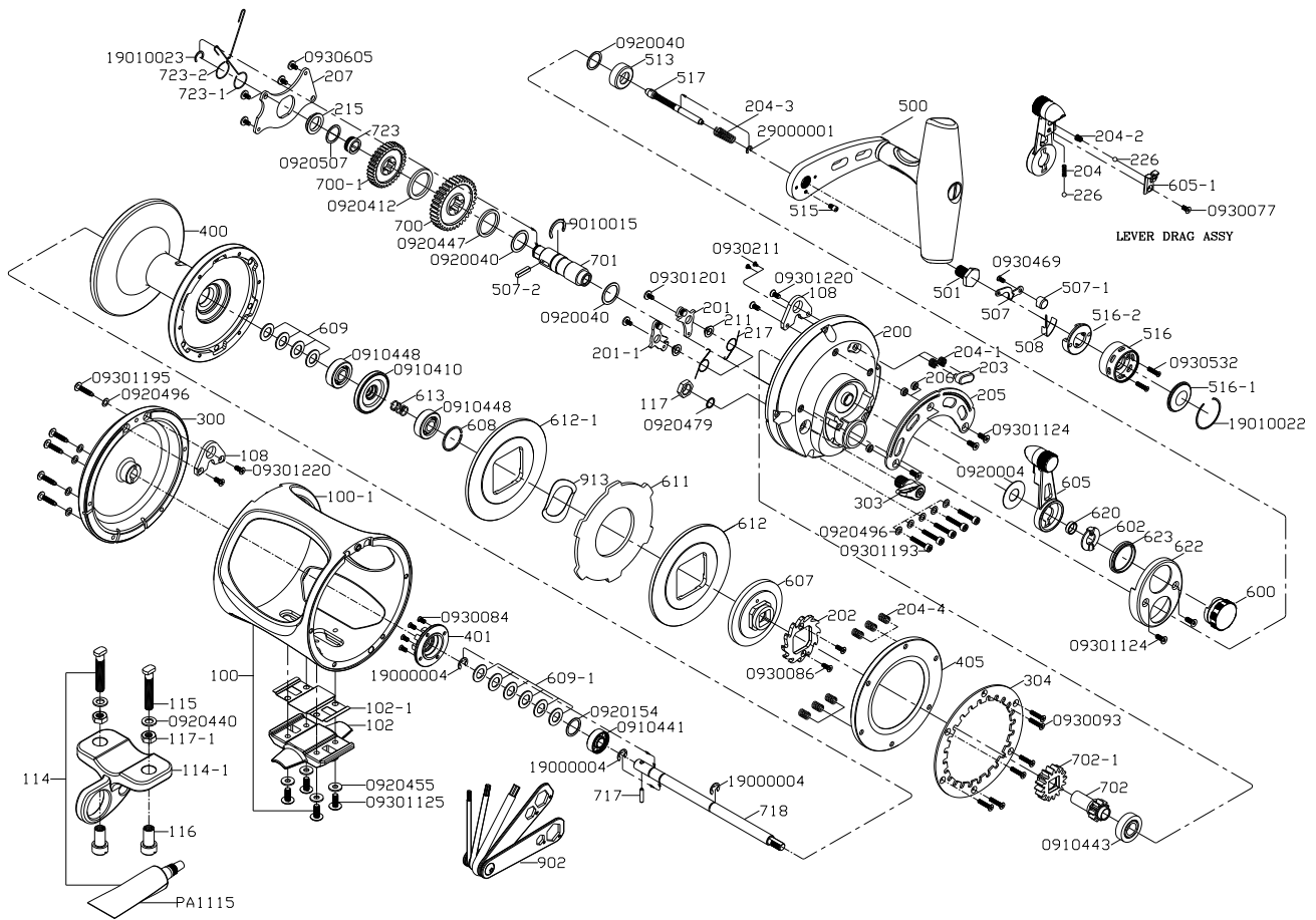
Makaira 50W-II PARTS LIST
