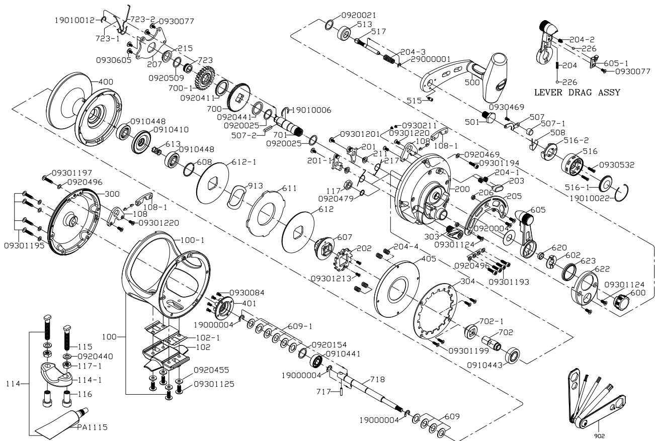
Makaira 20-II PARTS LIST
